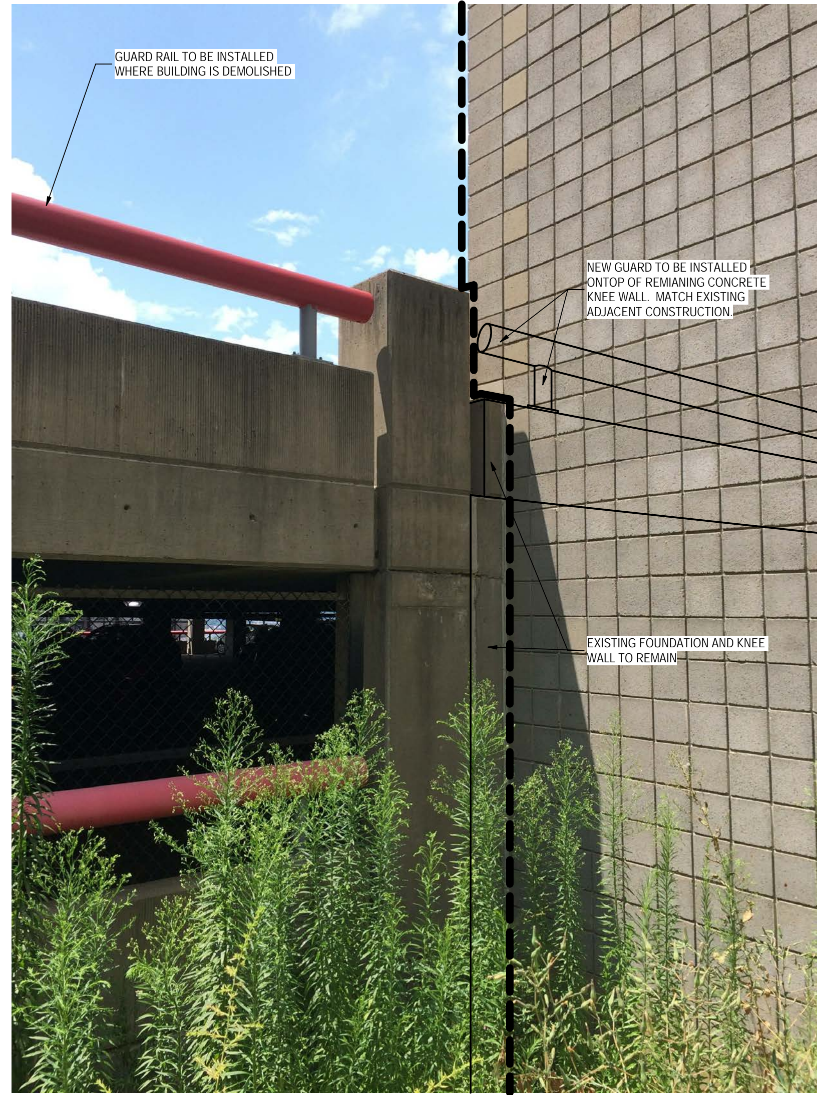
2 VIEW OF GUARD RAIL A105 1/4" = 1'-0"
