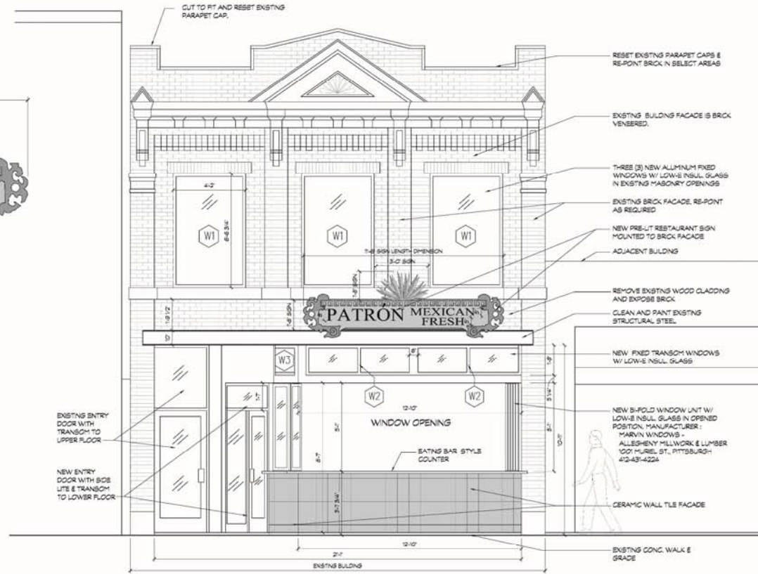
1 A3.1a BUILDING ELEVATION SCALE: 1/2" = 1'-0"
