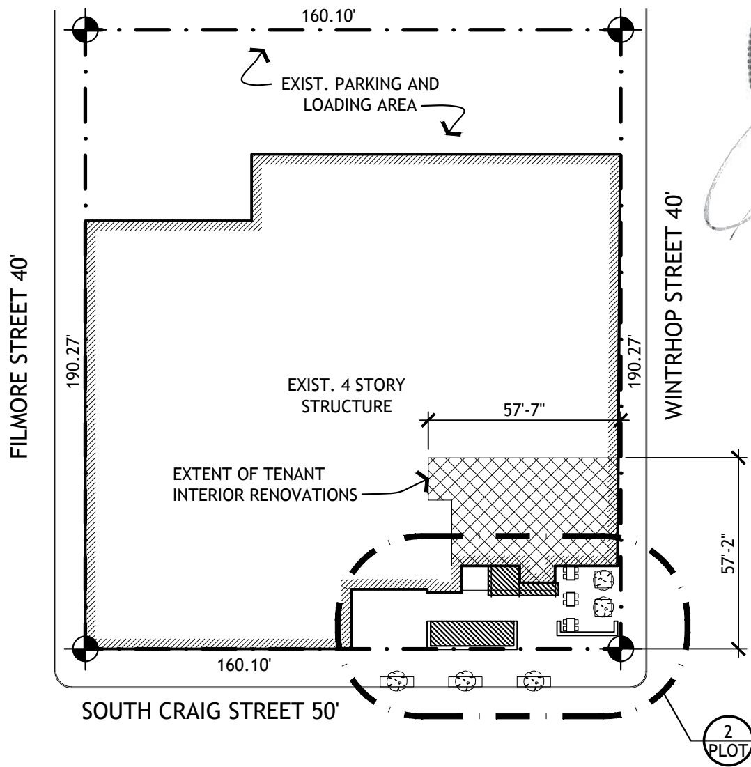
1 PLOT PLAN SCALE: 1" = 40'-0"
