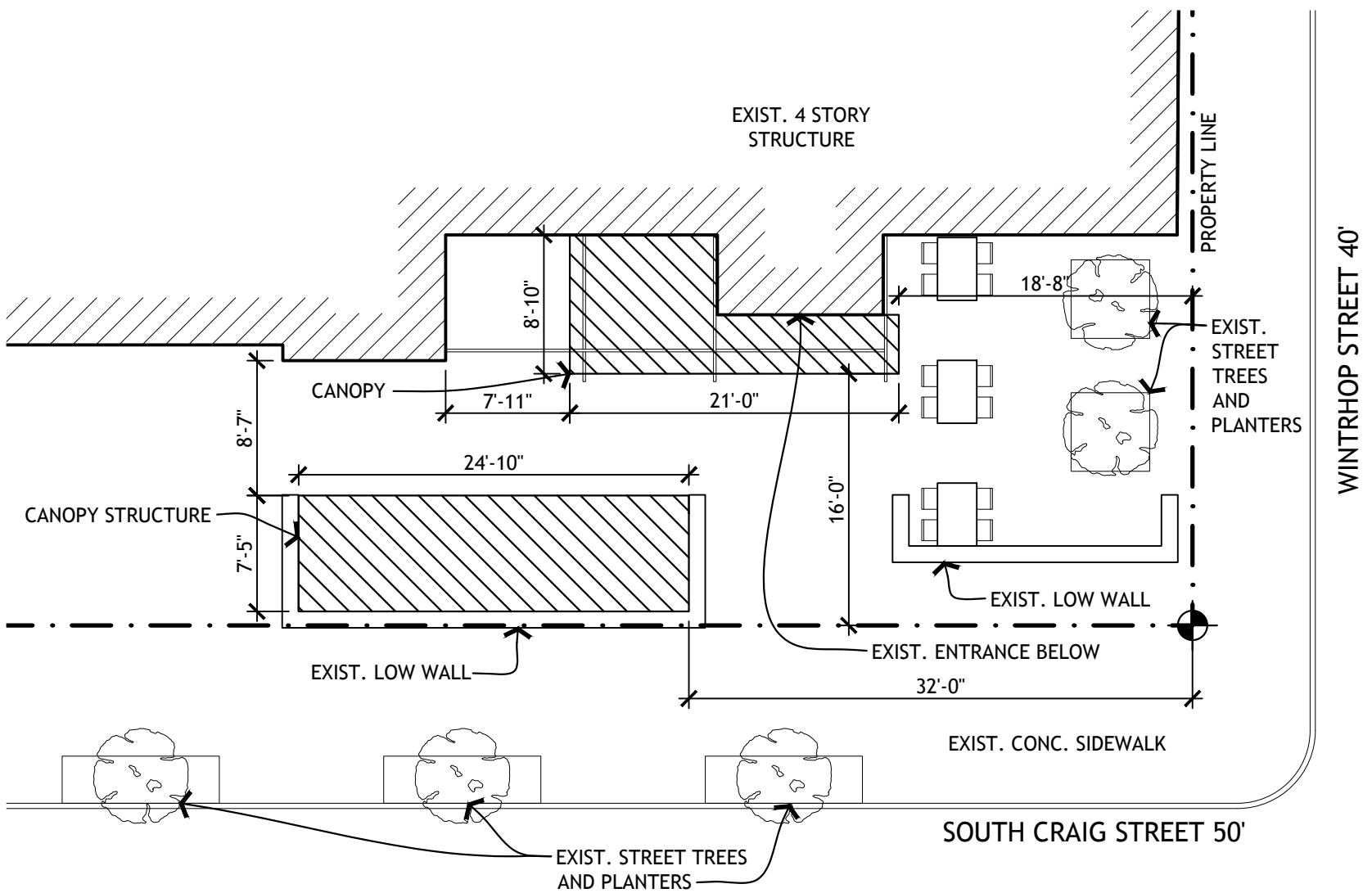
2 PLAN AT FRONT SCALE: 1" = 10'-0"
